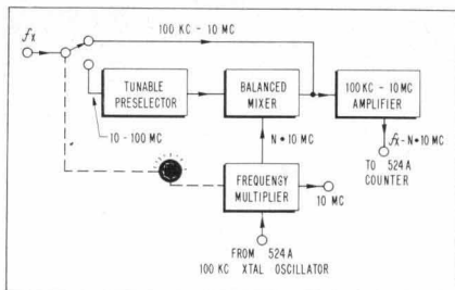
Fig. 2. Basic circuit arrangement of converter.
